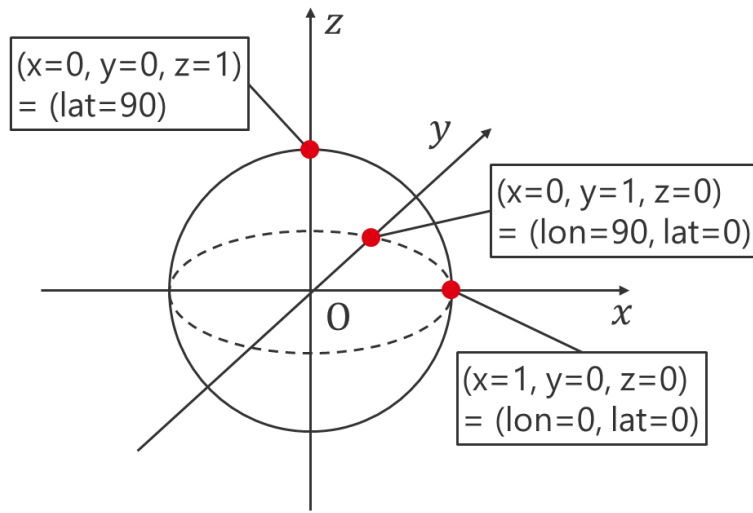
Figure 3-4 Cartesian coordinates in SPRING.
