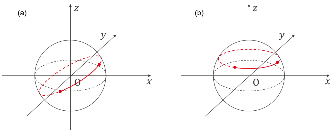
Figure 3-2 Great arc and small arc. (a) The red dashed line is the great circle, the red solid line is the great arc, and the red points are the edges of the arc. (b) The red dashed line is the small circle, the red solid line is the small arc, and the red points are the edges of the arc. Black dashed line is an intersection of the plane z=0 and the surface of sphere.
