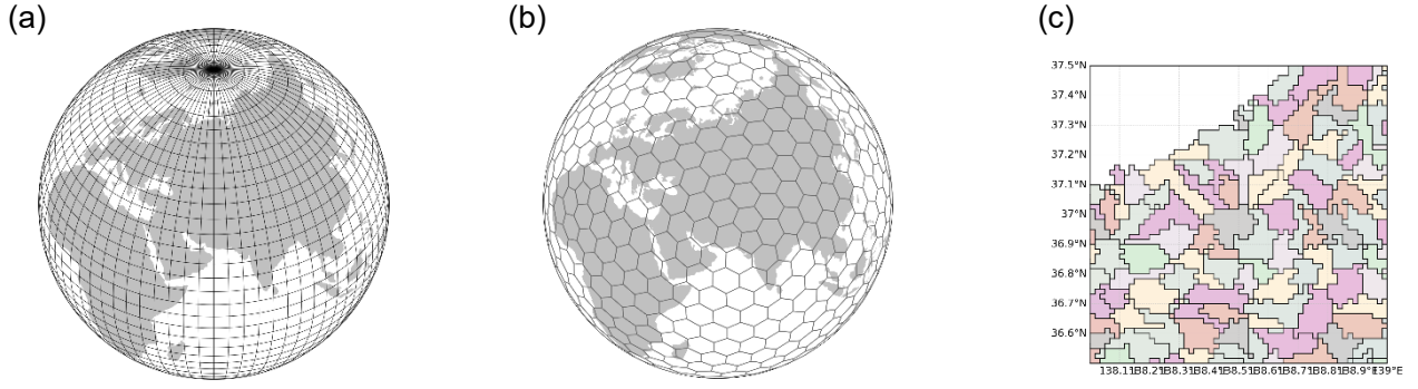
Figure 3-3 Examples of three types of meshes. (a) latlon mesh, (b) polygon mesh and (c) raster mesh.
