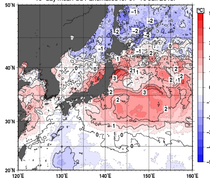
10-day mean SST anomalies for 01–10 Jul. 2018.
